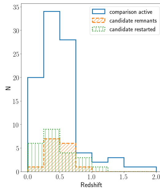
Fig. 4. Histogram showing redshift distribution of candidate restarted (green), remnant (orange) and active (blue) radio galaxies for the sources with an optical counterpart, see Sect. 4.2 for details.
