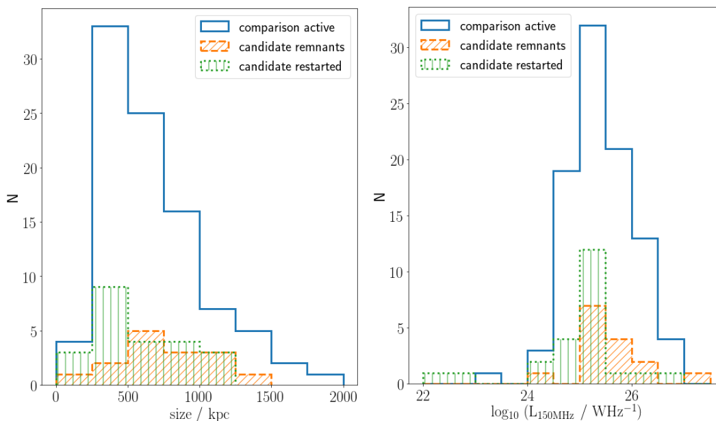
Fig. 7. Histogram showing linear sizes in kpc (left) and radio luminosity in \text{WHz}^{-1} at 150 MHz (right) of candidate restarted (green), candidate remnant (orange) and comparison active (blue) radio galaxies with optical identification from the SDSS or lower limit in redshift from WISE (see text for details).
