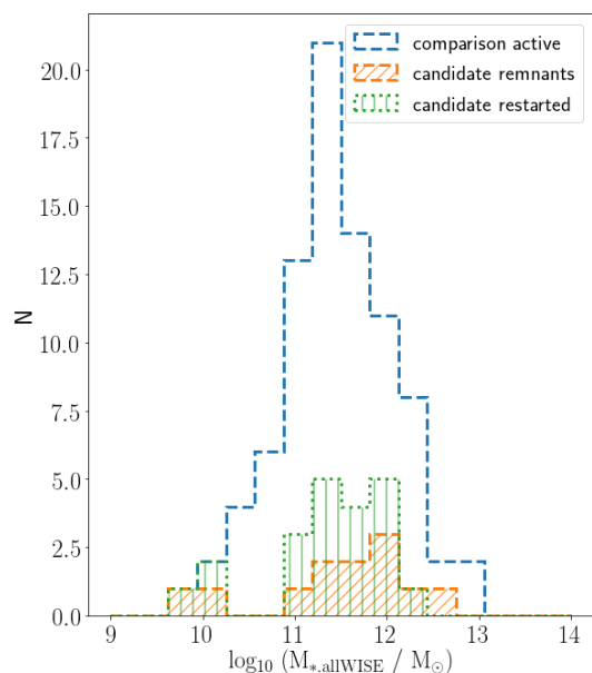
Fig. 6. Histogram showing stellar masses in solar masses of candidate restarted radio sources (green), remnant (orange) and comparison active (blue).
