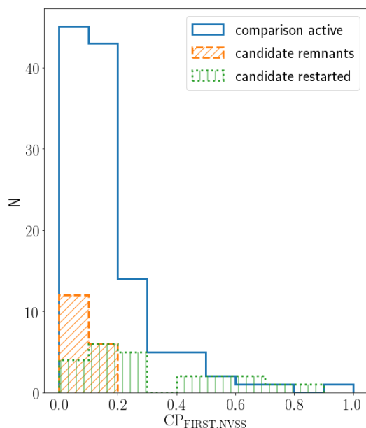
Fig. 3. Histogram showing the core prominence distribution of candidate restarted (green), candidate remnant (orange) mostly upper limits and comparison active (blue) radio galaxies. The restarted sample shown here includes all candidates selected with the different criteria, not only CP + low SB, see Sect. 4.3.
