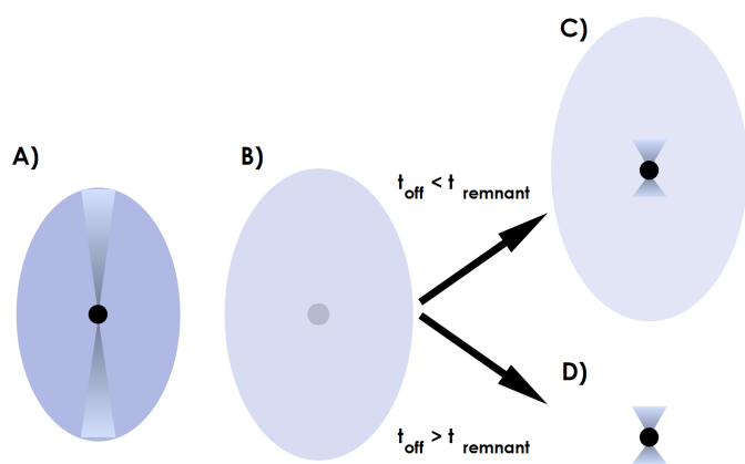
Fig. 1. Sketch of the life cycle of radio galaxies with different scenarios for the restarted phase. It shows an active galaxy (A) going through a remnant phase (B), and then through a restarted phase (C and D). Depending on the duration of the active phase with respect to the remnant fading time we can observe a restarted morphology (C) or a simple compact/young radio source (D).
