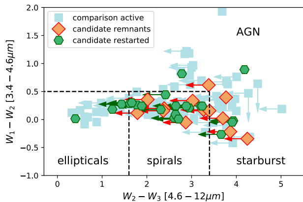
Fig. 5. WISE colour-colour diagram showing the sample of candidate remnant radio galaxies (orange diamonds), candidate restarted radio galaxies (green hexagons) and sample of active galaxies (blue squares). The upper limits are indicated as arrows. Classification following Mingo et al. (2016).
