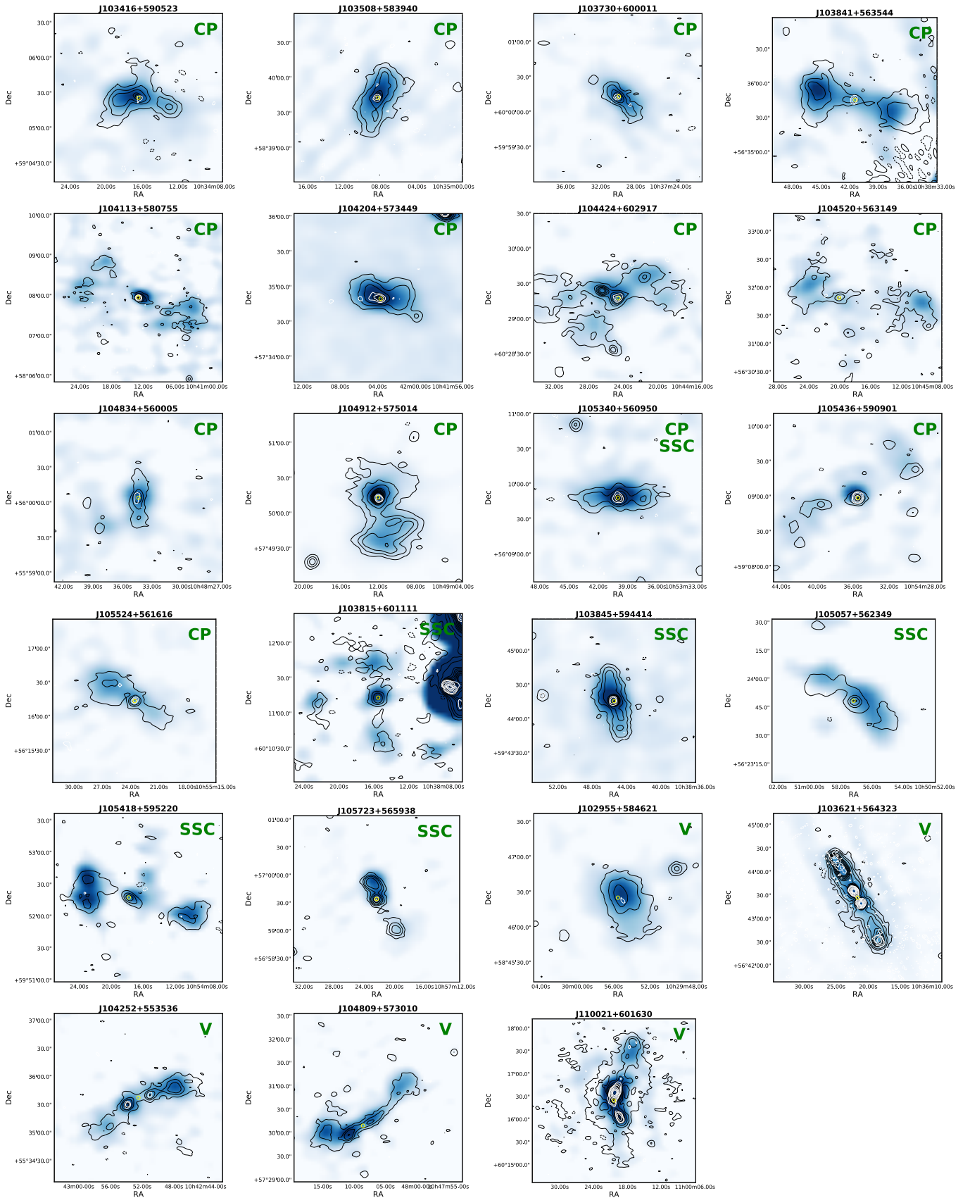
Fig. A.1. Candidate restarted radio galaxies selected on the basis of CP 1400 MHz and low surface brightness extended emission (see Sect. 4.3.1), steep spectrum of the inner region (see Sect. 4.3.2) or visual inspection (see Sect. 4.3.3). LOFAR radio contours ( -3, 3, 5, 10, 20, 30, 40, 50, 100, 150, 200 \times \sigma_{\text{local}} ) of the 6'' resolution map contours (black) and FIRST contours (white) are overlaid on the LOFAR 18'' resolution image. Position of the optical counterpart is noted with a yellow circle.
